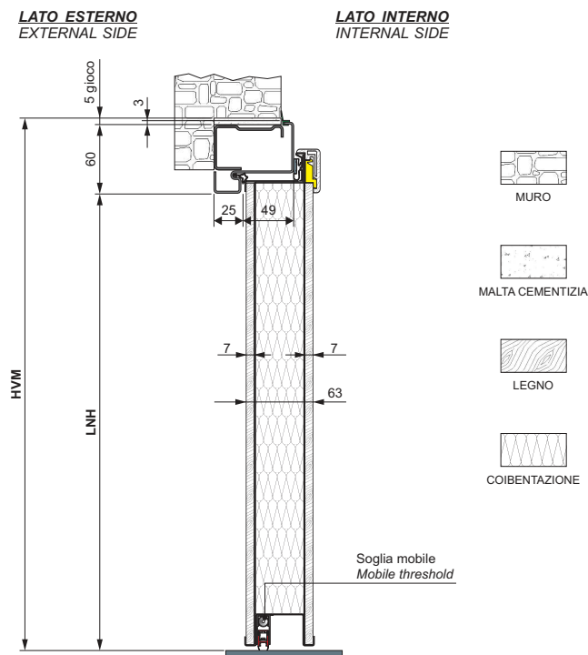
SCHEMA RINFORZI VISTI DI LATO REINFORCEMENT DIAGRAMS SEEN FROM SIDE
